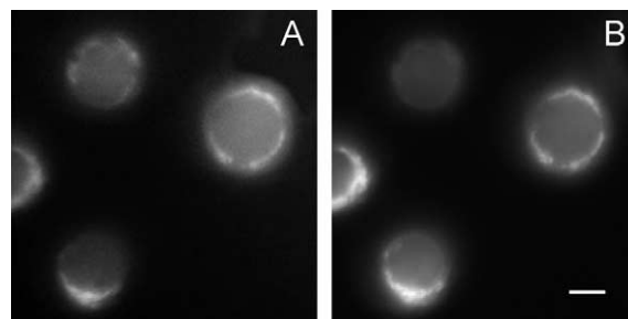
Fig. 2. Psoralen is localized to mitochondrial membrane. Jurkat cells were loaded with 50 \mu M psoralen (A) and 25 nM TMRM (B) and their fluorescence emission was visualized by fluorescence microscopy. The pattern of psoralen fluorescence closely matched that of TMRM. Scale bar = 5 \mu m.
